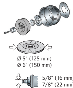
Type 6 and 11 Cup Wheels
