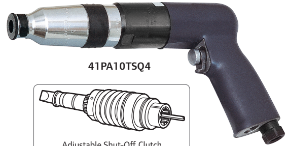
Adjustable Shut-Off Clutch
