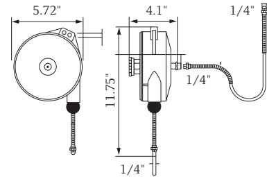
BHR Series
