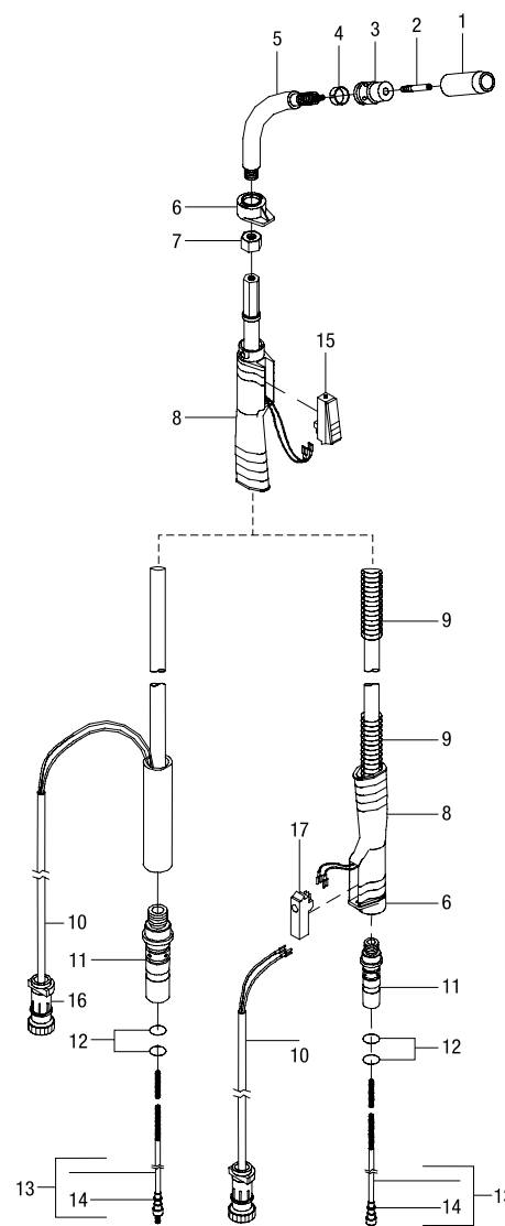
M-10 Gun
