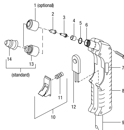
ICE-12C Torch
