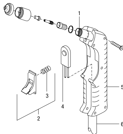
ICE-55C Torch
