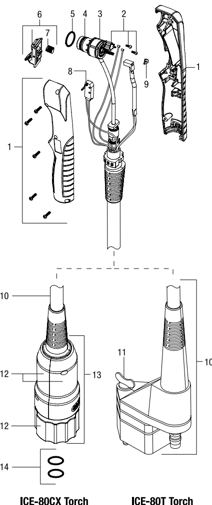
ICE-80CX Torch
