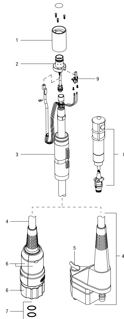
ICE-80CXM Torch
