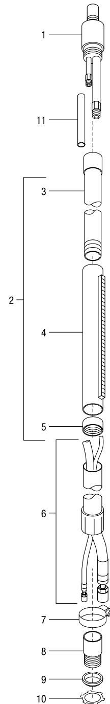
ICE-70M/ICE-100M Torch
