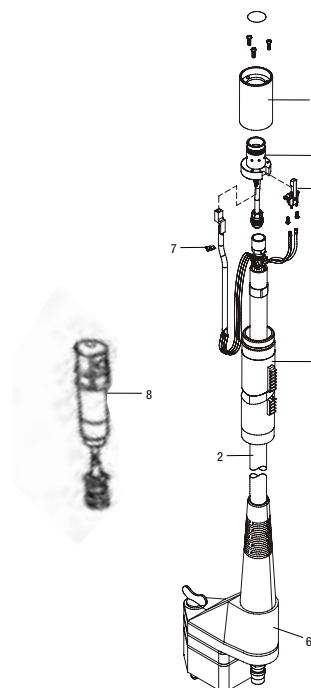
ICE-60TM Torch
