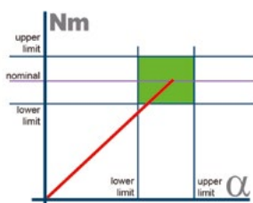
Torque & Angle Torque + Angle
